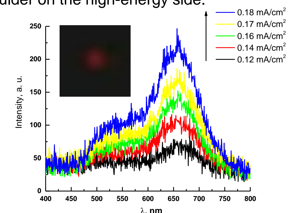
3 Room temperature EL spectra of our OLED under different injected currents. Inset shows a snapshot of light emission
