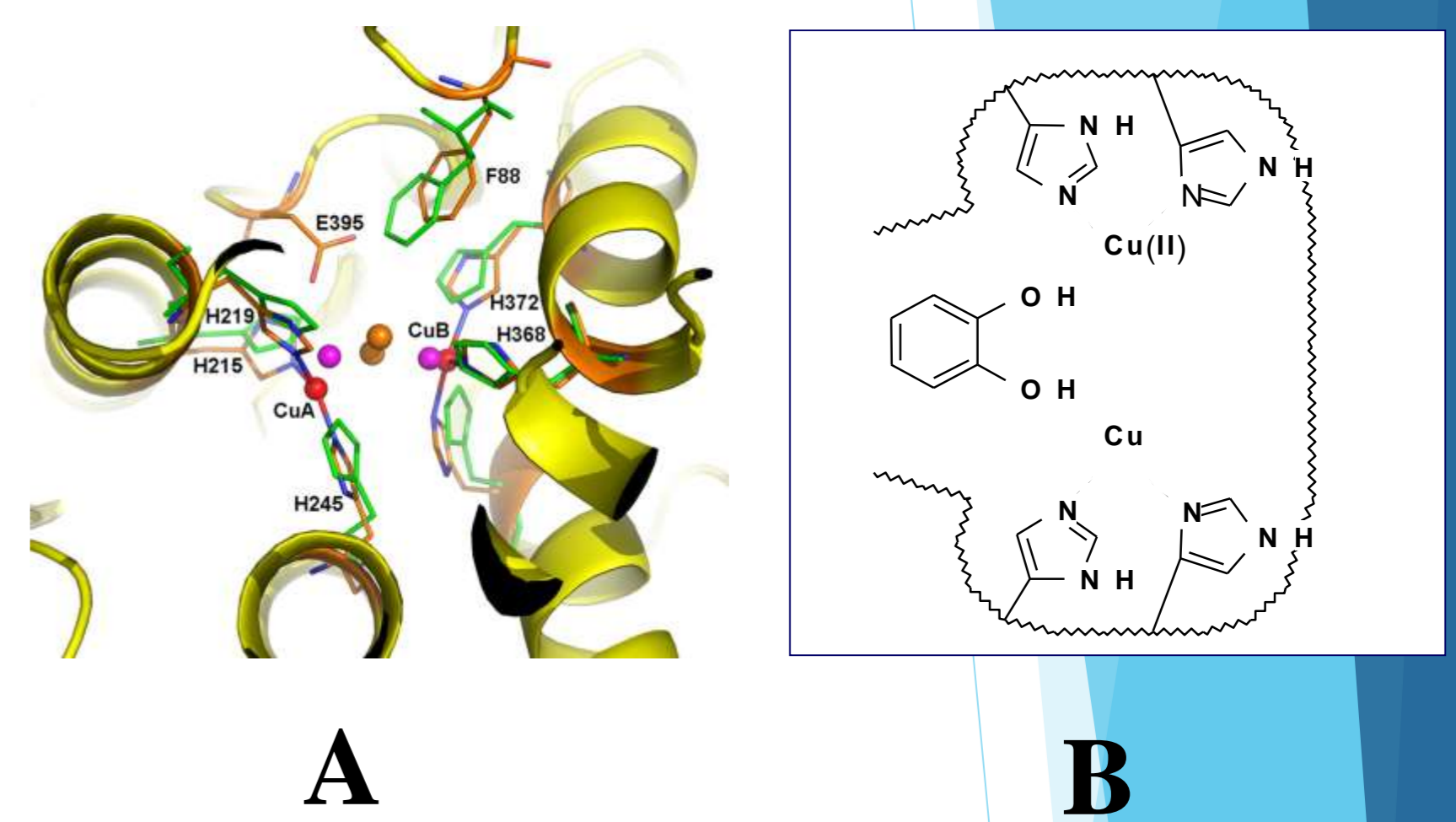
Fig.1. Possible structure of mammalian tyrosinase active site according to García-Borrón J.C. and Solano F., 2002 (A) and possible structure of the MIP with tyrosinase activity (B)
