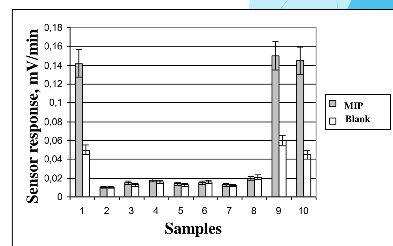
Fig.3. Responses of the o -hydroxyphenol-selective sensor in response to addition of 1 mM of o -hydroxyphenol (1), phenol (2), 2-nitrophenol (3), 4-nitrophenol (4), o -cresol (5), p -cresol (6), 2-methoxyphenol (7), m -hydroxyphenol (8), 2-(3,4)-dihydroxyphenyl)-ethylamine (9), and 1,2,3-trihydroxybenzene (10) as analytes
